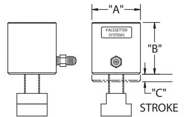
Models 241/261/281
