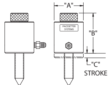
Models 245/265/285
