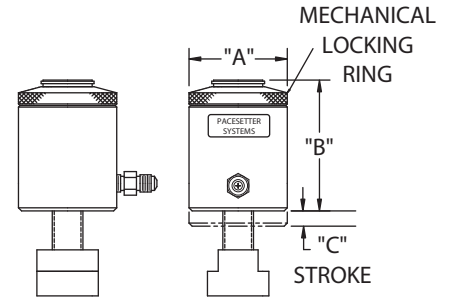
Models 240/260/280
